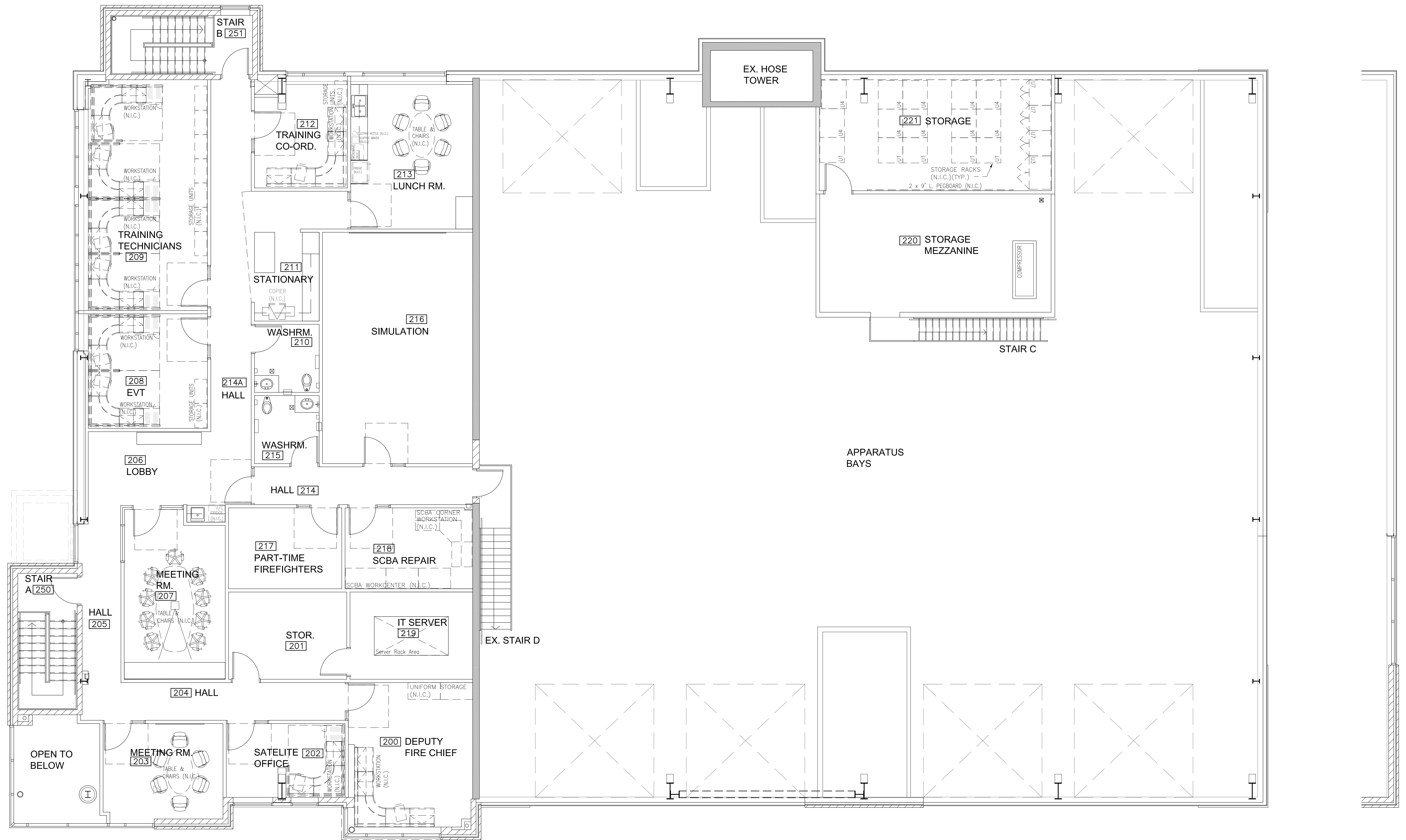
SECOND FLOOR PLAN BUILDING REHABILITATION OF FIRE STATION No. 1 MILTON, ONTARIO N.T.S.
